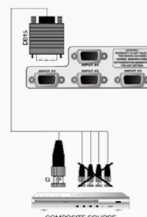
COMPOSITE SOURCE
